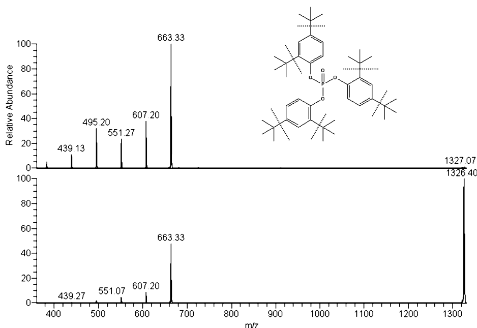
Figure 5. MS-MS spectra for the ion at m/z 1325, identified as oxidized Irgafos 168. Several peaks with 56 amu ( \text{C}_4\text{H}_8 ) difference could be observed ( m/z 383, 439, 495, 551, 607, 663) corresponding to neutral losses of the tert -butyl groups, each followed by proton transfer. (Top) After application of 40% collision energy. (Bottom) After application of 20% collision energy.
