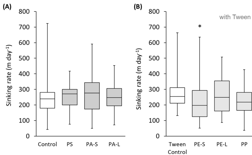
Fig. 3. Box-and-whisker plot showing sinking rates (m day -1 ) of mussel faeces, with and without microplastics, in seawater: (A) Exposure to neutrally buoyant PS, PA-S and PA-L; (B) Exposure to low density PE-S, PE-L and PP with 0.01% Tween surfactant to facilitate immersion in seawater. * denotes statistical significance from relevant control (Kruskal-Wallis, P = 0.04).
