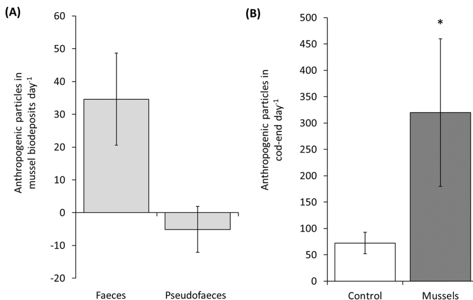
Fig. 5. Microplastics collected via mussel deployment systems in an urban marina. (A) Comparison of microplastic concentrations in mussel faeces and pseudofaeces in flowthrough systems. (B) Microplastics samples from cod-end of sub-surface system for control and mussel treatments. Data shown as mean \pm standard error, normalised to 5.0 kg mussels; * denotes statistical significance from the control (t-test, P < 0.05 ).
