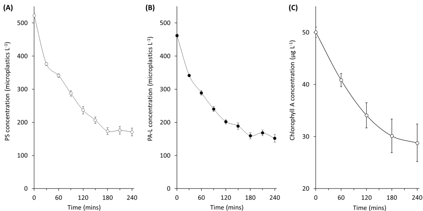
Fig. 2. Concentrations of (A) PS and (B) PA-L (microplastics L -1 ), and (C) Chlorophyll A (µg L -1 ) in flume tank over a 4-hour period following exposure to mussels ( Mytilus edulis ). Data shown as mean ± standard error, normalised to 5.0 kg mussels.
