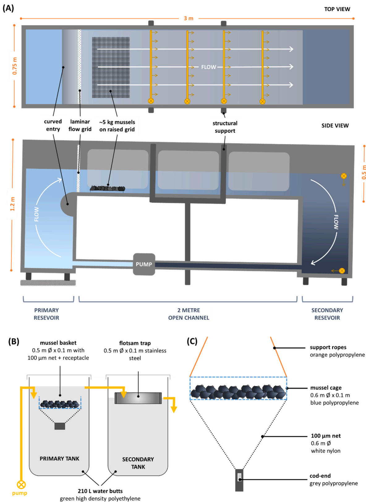
Fig. 1. Schematics for the flume tank (laboratory experiment) and mussel deployment systems (field trials). (A) The flume tank housed mussels in an open channel with continuous \sim 0.2 \text{ m s}^{-1} flow generated by a 1.5 HP pump. Smaller in-line pumps (yellow circles; yellow arrows denote direction of flow) were positioned within the tank to prevent microplastics settling out; along open channel, the in-line pumps were connected to piping to direct water flow evenly across the base of the chamber. Three polycarbonate windows in the side of the 2 m long open channel permitted observation of mussels and biodeposit formation. (B) Flowthrough system in which natural seawater is pumped into the primary tank containing a basket of mussels; a 100 \mu m mesh net directs sinking faeces into a receptacle, while floating pseudofaeces, are directed into a flotsam trap in the secondary tank. Yellow arrows indicate water flow via piping. (C) Sub-surface system in which caged mussels are suspended in water-column, with a 100 \mu m mesh net and cod-end positioned beneath to capture microplastic-laden faeces.
