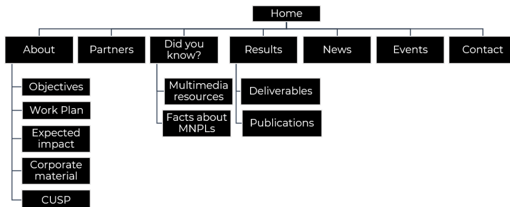
Figure 4. Website map.
