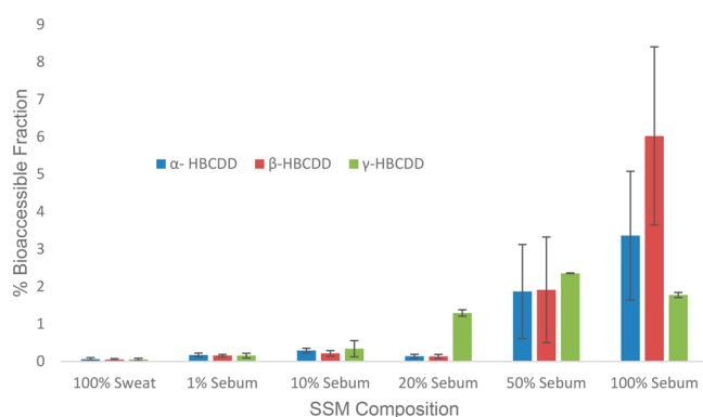
Figure 4. Influence of SSM composition on the bioaccessibility of HBCDD in polystyrene MPs.
