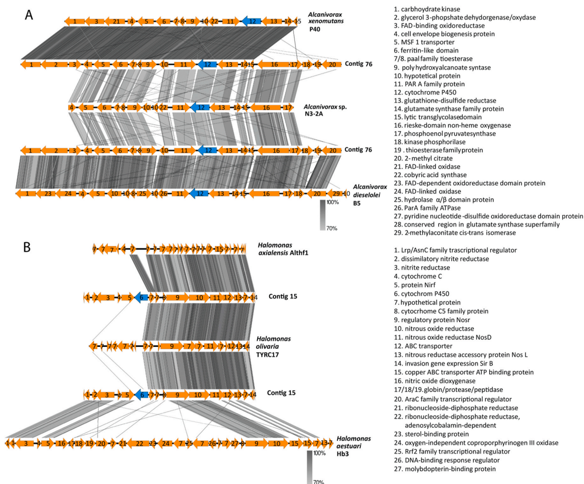
Fig. 5. A–B Comparative genomics of genetic regions for peripheral pathways for hydrocarbon degradation with cytochrome P450 (CYP450).A) Comparison of contig 76 from A. xenomutans strain SRM1 MAG (containing the ORF 12 encoding for CYP450) with three closest sequences from the NCBI database. In the right, the complete list of genes encoded within contig 76 (ORFs 1–20) and those encoded by the 3 other reference genomes (ORFs 21–29). B) Comparison of contig 15 from H. alkaliantarctica strain SRM2 MAG (containing the ORF 6 encoding for CYP450) with three closest sequences from the NCBI database. In the right, the complete list of genes encoded within contig 15 (ORFs 1–14) and those encoded by the 3 other reference genomes (ORFs 15–27).
