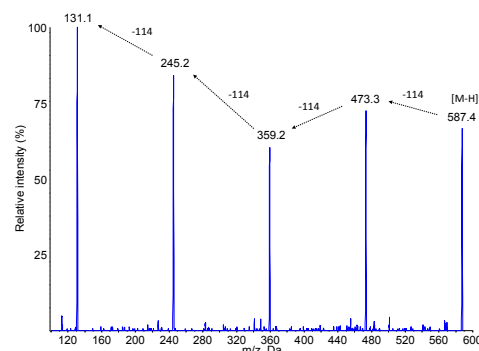
Figure 6: Negative electrospray ionization fragmentation mass spectra of the [M-H]^- pseudo-pseudo molecular ion of compound PCL7, namely the PCL pentamer.
