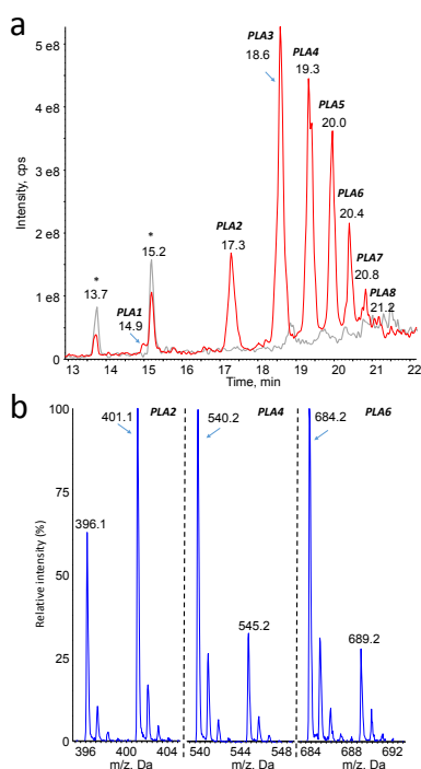
Figure 1: a) HPLC-MS1 chromatogram recorded upon analysis of aged 150 nm PLA particles before (grey) and after (red) aging at 55°C. Peaks labelled * were present before aging. Detection was made in positive electrospray ionization with the spectrometer used as a linear ion trap (mass range 50-1000); b) mass spectra centered around the [M+NH_4]^+ and [M+Na]^+ pseudo-molecular ions for the compounds eluting in peaks PLA2, PLA4 and PLA6.
