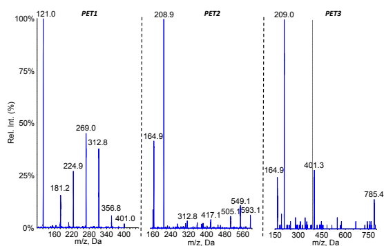
Figure 8: Negative electrospray ionization fragmentation mass spectra of the [M-H] - pseudo-pseudo molecular ion of compound PET1, PET2 and PET3, namely the dimer, trimer and tetramer of PET, respectively.
