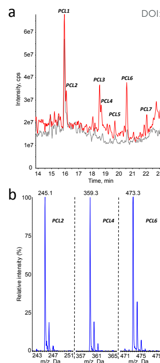
Figure 5: a) HPLC-MS1 chromatogram recorded upon analysis of aged 200 nm PCL particles before (grey) and after (red) aging. Detection was made in negative electrospray ionization with the spectrometer used as a linear ion trap (mass range 50-1000); b) mass spectra centred around the [M-H]^- pseudo-molecular ions for the compounds eluting in peaks PCL2, PCL4 and PCL6.
