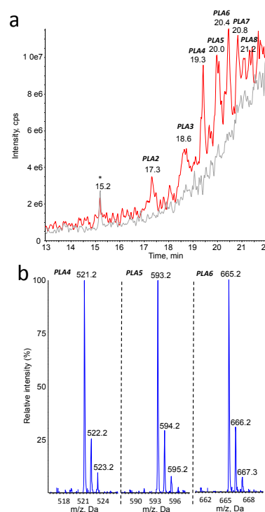
Figure 2: a) HPLC-MS1 chromatogram recorded upon analysis of aged 150 nm PLA particles before (grey) and after (red) aging at 55°C. Peaks labelled * were present before aging. Detection was made in negative electrospray ionization with the spectrometer used as a linear ion trap (mass range 50-1000); b) mass spectra centered around the [M-H]^- pseudo-molecular ions for the compounds eluting in peaks PLA2, PLA4 and PLA6.
