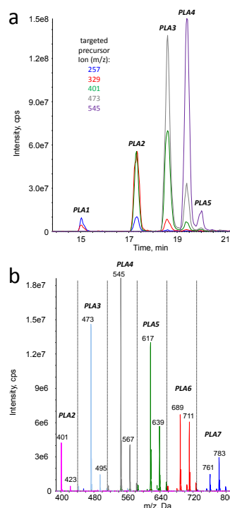
Figure 4: a) Precursor ion scan analysis of aged PLA with positive electrospray ionization. The targeted ions were those identified by MS2 analyses and are listed on the figure; b) Neutral loss analysis of aged PLA with positive electrospray ionization. The monitored loss was -72. The figure shows the m/z ratio of the pseudo-molecular ions detected under each chromatographic peak.
