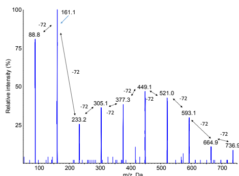
Figure 3: Negative electrospray ionization fragmentation mass spectra of the [M-H]^- pseudo-pseudo molecular ion of compound PLA7, namely the PLA decamer.
